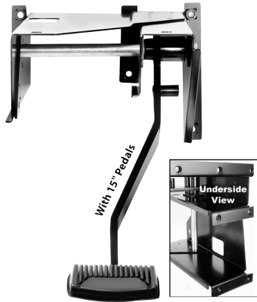
3771 1966-77 Manual Brake Pedal Assembly
